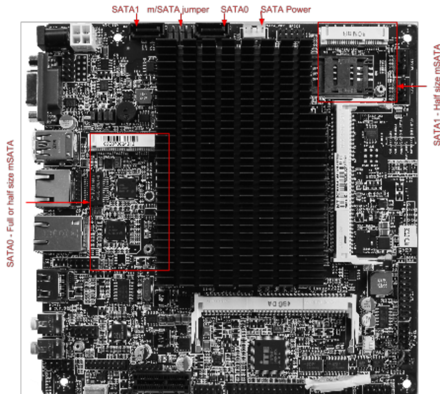
Figure 3: SATA and mSATA
