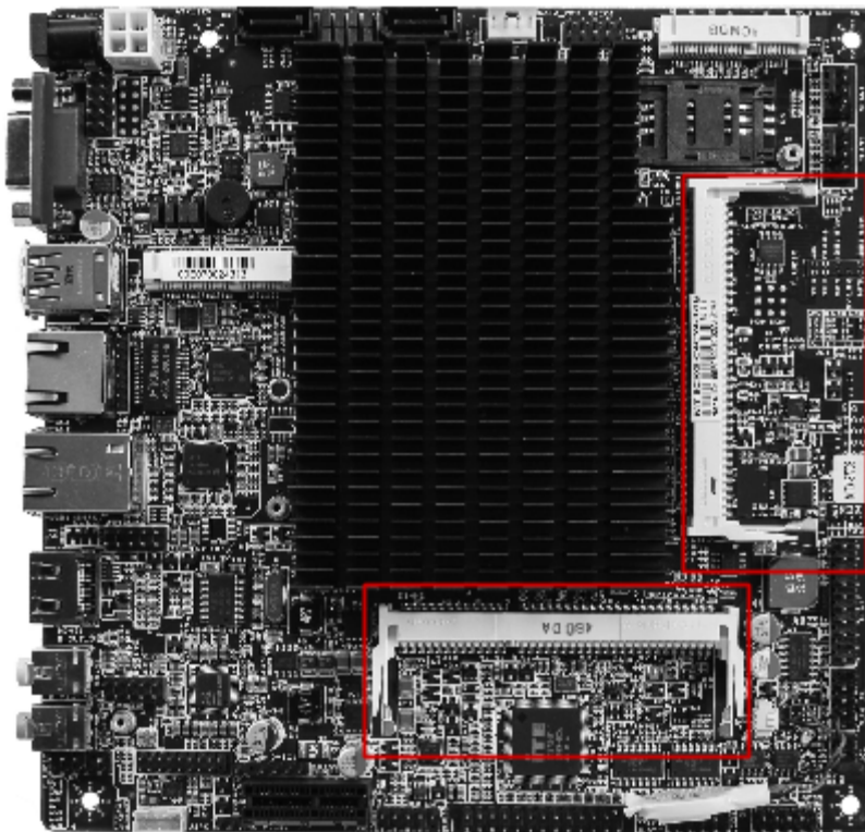
Figure 1: DIMM
