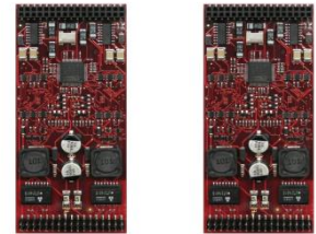
2 2BRI/2FXS Modules
